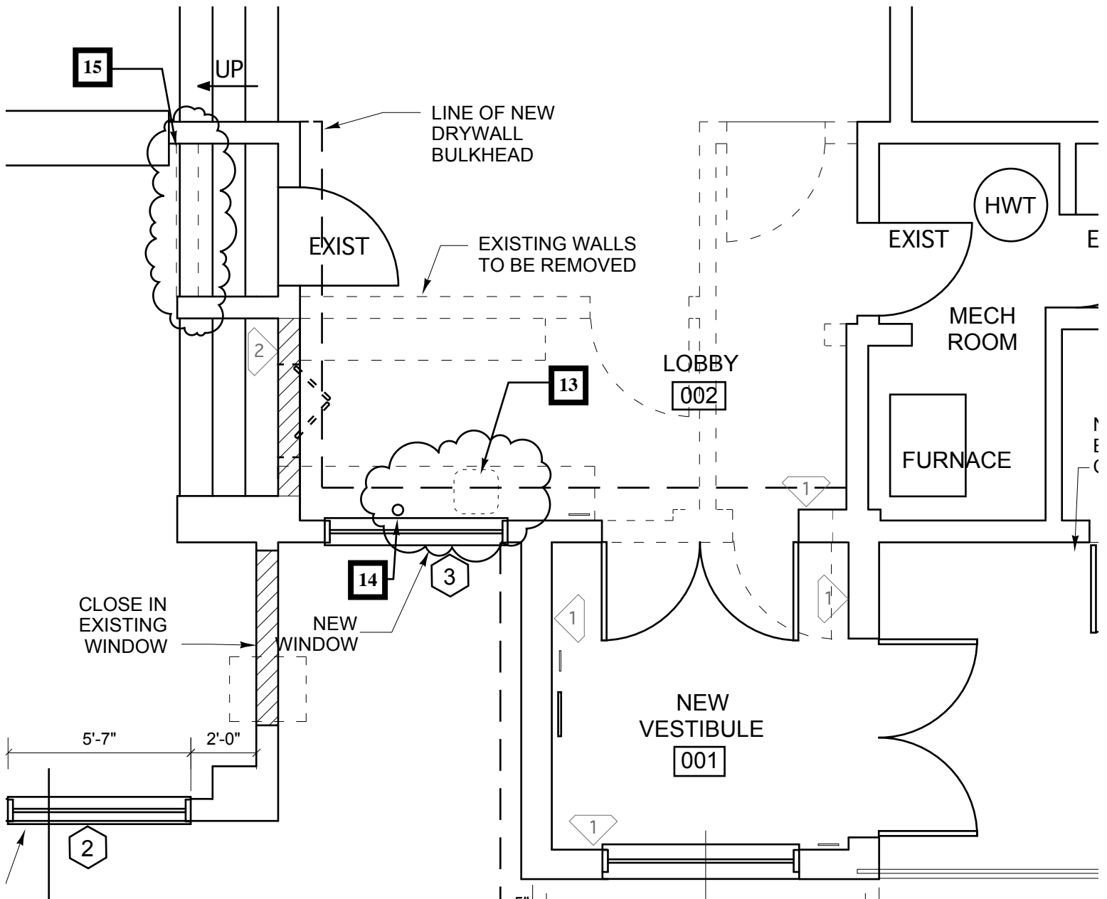
1 ENLARGED PARTIAL PLAN AR-1 SCALE: 1/4" = 1' - 0"
